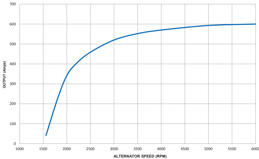
PERFORMANCE CURVE AB210R - 600A (@25°C Ambient & 100% Load)
